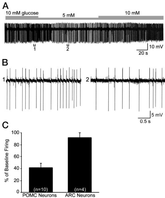
FIG. 9. POMC neurons are glucose responsive. A, Reduction in extracellular concentrations of glucose from 10 mM to 5 mM significantly decreased the firing rate of a POMC neuron recorded in the cell-attached mode. The cell fully recovered to its original baseline firing rate. B, Expansion of chart record in A shows that the spontaneous firing rate decreased from 6 Hz (bracket 1) to about 3 Hz (bracket 2) or a 50% reduction in firing. C, Summary of the decrease in the spontaneous firing rate in POMC vs. unidentified, adjacent arcuate neurons following a reduction in the glucose concentration from 10 to 5 mM. Bars represent the mean, and lines 1 SEM of the baseline firing rate. Eighty percent (10 of 12) of the POMC neurons were inhibited by a reduction in glucose concentration.
