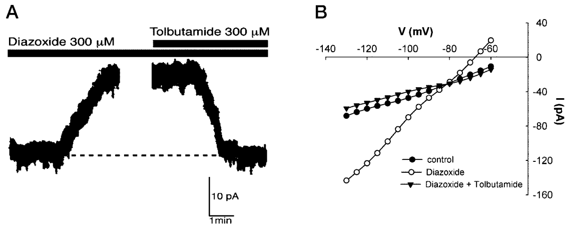
FIG. 5. Female mouse POMC neurons respond to the K_{ATP} channel opener diazoxide. A, In the presence of TTX, a POMC neuron responded to the K_{ATP} channel opener diazoxide ( 300 \mu\text{M} ) with 20 pA outward current. This effect was reversed by the sulfonylurea tolbutamide ( 300 \mu\text{M} ). The break in the recording trace indicates where I/V data were obtained. V_{\text{hold}} = -60 \text{ mV} (resting V_m = -50 \text{ mV} ). B, The prediazoxide, postdiazoxide, and postdiazoxide + tolbutamide current-voltage relationships from the POMC neuron in panel A. The reversal potential for the outward current was close to the predicted equilibrium potential for potassium ( E_{\text{diazoxide}} = -85 \text{ mV} ).
