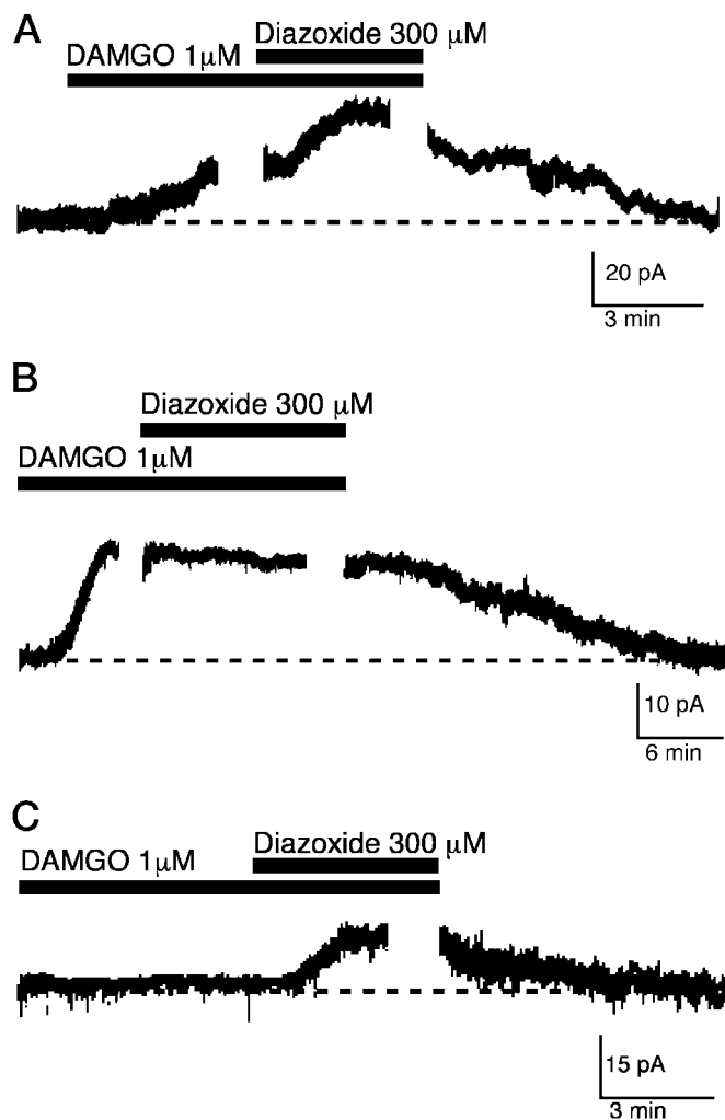
FIG. 7. Three populations of POMC neurons based on their response to DAMGO and diazoxide. A, The effects of DAMGO and diazoxide were additive in the majority of female mouse POMC neurons. Diazoxide (300 \mu\text{M} ) produced an additional 22-pA outward current when coperfused with DAMGO (1 \mu\text{M} ), which generated a maximal outward current of 18 pA in the presence of 1 \mu\text{M} TTX. The breaks in the recording trace indicates points where current/voltage data were obtained. V_{\text{hold}} = -60 mV (resting V_m = -54 mV). B, A subpopulation of female POMC neurons responded to DAMGO only. Coperfusion of diazoxide (300 \mu\text{M} ) did not augment to maximal outward current produced by 1 \mu\text{M} DAMGO (25 pA) in the presence of 1 \mu\text{M} TTX. The breaks in the recording trace indicates points where current/voltage data were obtained. V_{\text{hold}} = -60 mV (resting V_m = -51 mV). C, A subpopulation of female POMC neurons responded to diazoxide only. Diazoxide (300 \mu\text{M} ) induced maximal outward current of 15 pA in the presence of 1 \mu\text{M} TTX following the application of 1 \mu\text{M} DAMGO, which had no effect in this POMC neuron. The break in the recording trace indicates when current/voltage data were obtained. V_{\text{hold}} = -60 mV (resting V_m = -57 mV).
