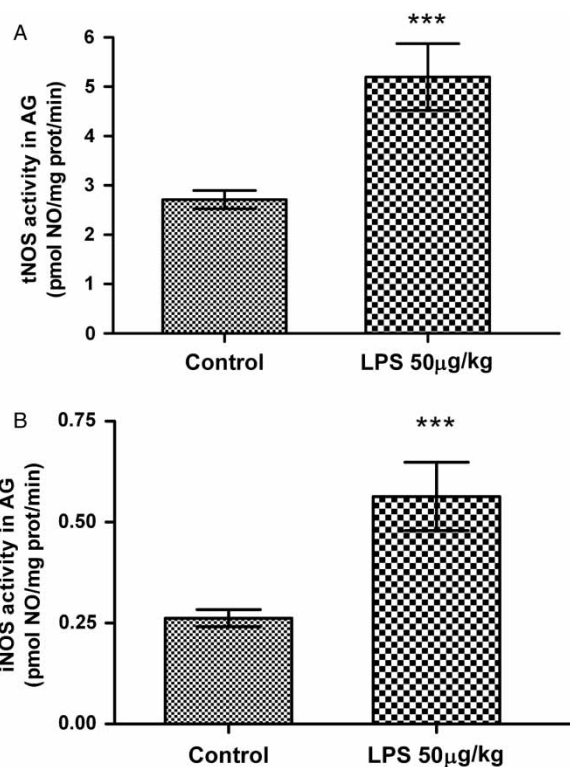
Figure 4. Effect of LPS (50 µg/kg, i.p.) on (A) tNOS and (B) iNOS activity in the adrenal gland (AG). Values represent mean ± SEM ( n = 6-8 rats per group). Data were evaluated by Student's t -test. *** p < 0.001 vs. control group.
