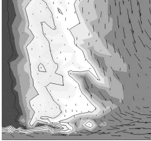
Figure 4. Zoom on the solidification front for Sn-5wt%Pb at 100s with THERCAST
