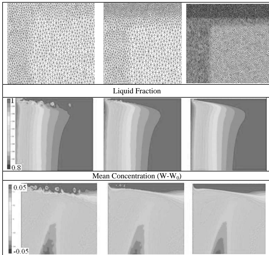
Figure 7. Liquid fraction and mean concentration at 10s for the Pb-48wt%Sn alloy on three different meshes
