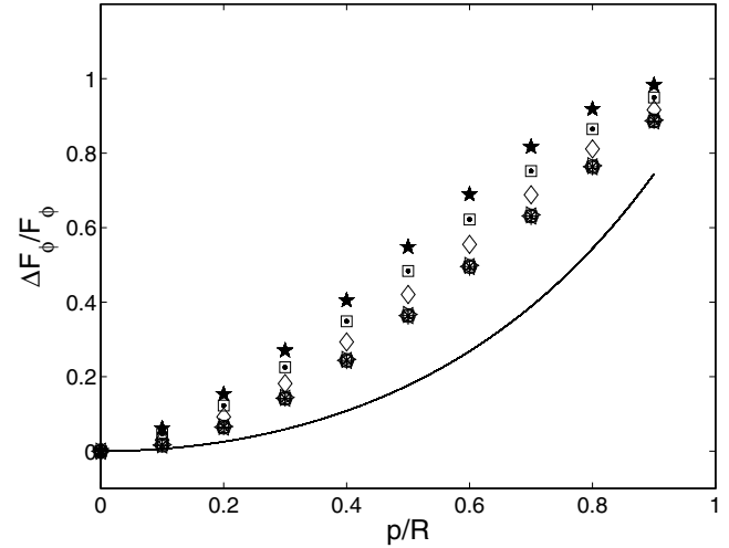
Fig. 10. Idem as Fig. 8 but for F_\phi/L values.
