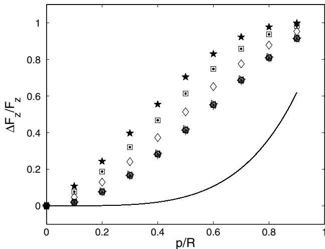
Fig. 9. Idem as Fig. 8 but for F_z values.
