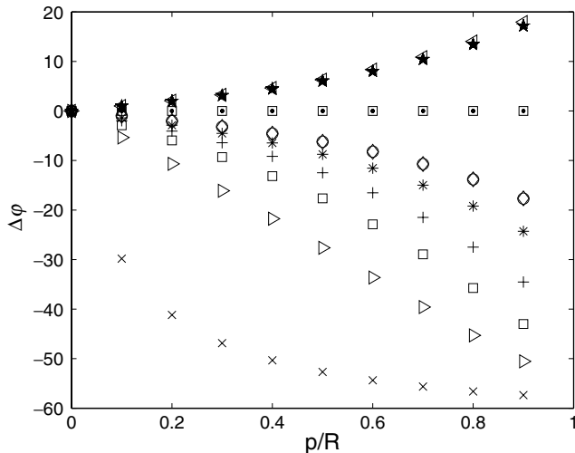
Fig. 4. Idem Fig. 3 but showing the difference in \varphi ( \Delta\varphi = \varphi - \varphi_{MV} ).
