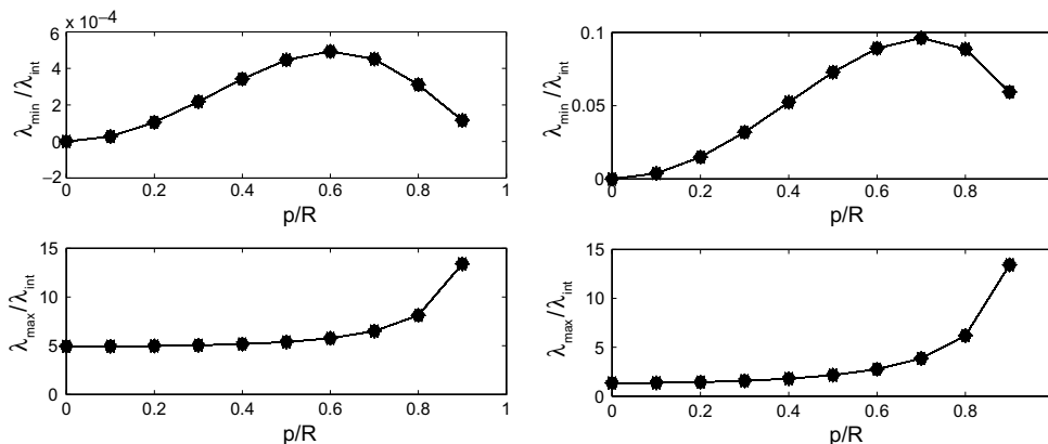
Fig. 1. Left: upper (lower) panel shows the ratio between the minimum and intermediate (maximum and intermediate) eigenvalues from MV (using m_{ij} ) for the set of generated MCs as a function of p in units of the MC radius. Right: upper (lower) panel shows the ratios but now using the matrix M_{ij} , where we take \mathbf{v}^k = \mathbf{b}^k for the set of generated MCs.
