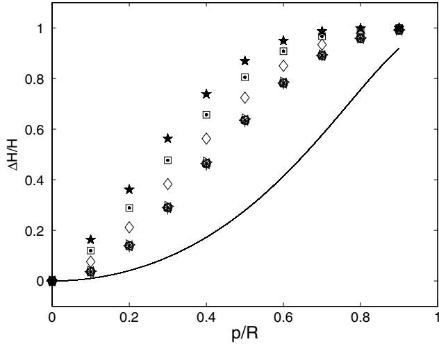
Fig. 8. Difference between the theoretical and estimated values (using MV) of the magnetic helicity, divided by the theoretical value, \Delta H/H = (H - H^{MV})/H , as a function of p/R . The symbols for different orientations are given as in Fig. 3. Solid line corresponds to H^{MV} computed with the values for B_0 and \alpha used to generate the synthetic MCs, B_0 (=20 \text{ nT}) and \alpha (=24 \text{ AU}^{-1}) , but considering the radius \sqrt{(R^2 - p^2)} .
