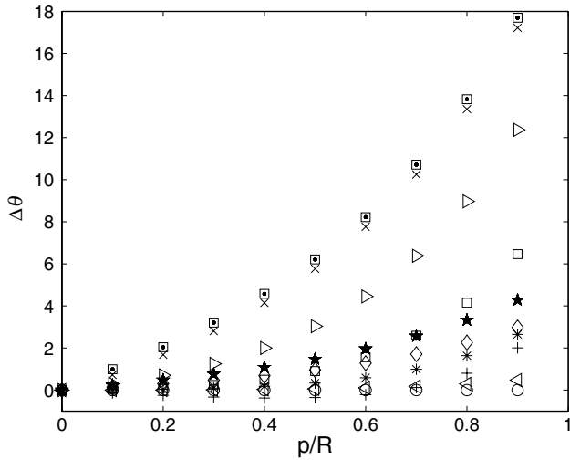
Fig. 3. Bias from Minimum Variance in \theta ( \Delta\theta = \theta - \theta_{MV} ) in function of p in units of the radius. Different orientations of the synthetic clouds are represented by (\theta, \varphi) = * (45, 90), \times (89, 120), + (60, 80), \circ (0, 90), \square (70, 90), \diamond (10, 130), \star (5, 200), \square (30, 180), \triangleleft (10, 270), \triangleright (80, 105).
