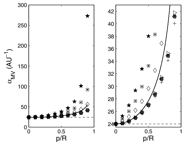
Fig. 7. \alpha_{MV} as a function of p/R . Dashed line corresponds to the value set to generate the synthetic clouds ( \alpha = 24 \text{ AU}^{-1} ). The symbols for different orientations are given as in Fig. 3. Solid line shows \alpha = 24 \text{ AU}^{-1}/\sqrt{1 - (p/R)^2} . The left panel shows the full set of clouds, while the right panel shows a zoom.
