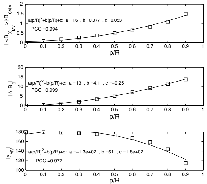
Fig. 5. Upper panel: |\langle B_{X_{MV}} \rangle|/B_{0MV} . Middle panel: \Delta B_0 = B_0 - B_{0MV} . Lower panel: absolute value of the rotation angle of \mathbf{B} in the plane of maximum variance ( |\gamma_{MV}| ). All the quantities are plotted, in function of p in units of the radius. Their quadratic regression curves are added.
