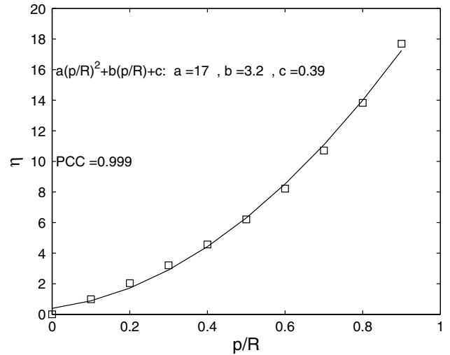
Fig. 2. Angle \eta between the generated cloud axis ( \hat{Z}_{\text{cloud}} ) and the one obtained by MV (squares) as a function of p in units of the MC radius together with the quadratic regression curve (solid line).
