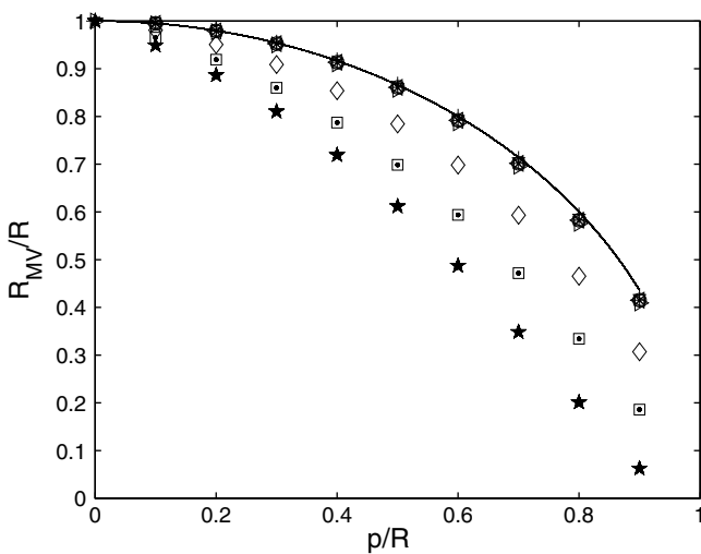
Fig. 6. R_{MV} in units of the synthetic radius R (= 0.1 \text{ AU}) as a function of p/R . Solid line corresponds to the small expected radius (because of the assumption p = 0 ) computed from the orientations of the synthetic MCs. Symbols are given as in Fig. 3.
