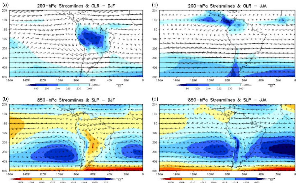
Figure 1. Mean (1979–2008) 200-hPa wind vector and outgoing longwave radiation (OLR) (top) and 850-hPa wind vector and sea level pressure (SLP) (bottom), for DJF and JJA. Units are \text{W m}^{-2} for OLR and hPa for SLP. Circulation data are derived from the NCEP/NCAR Reanalysis. This figure is available in colour online at wileyonlinelibrary.com/journal/joc
