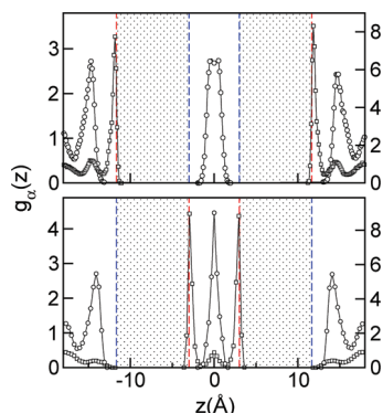
Figure 2. Density fields associated to W-oxygen (squares, right axis) and A-central-carbon sites (circles, left axis) for d = 6 \text{ \AA} . The results shown in the top (bottom) panel correspond to the PHO-PHO (PHI-PHI) arrangement. The shaded areas correspond to the volume excluded by the plates. Hydrophobic (hydrophilic) silica interfaces are rendered in blue (red).
