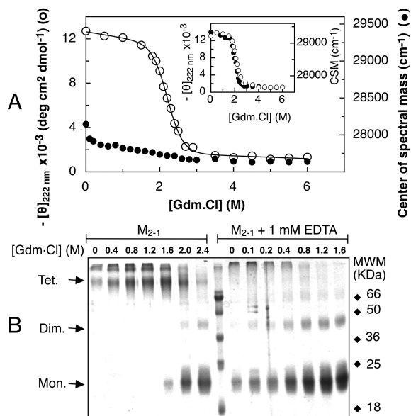
Figure 5. Gdm-Cl equilibrium unfolding of apo-M 2-1 at pH 7.0. (A) Apo-M 2-1 equilibrium unfolding transition followed by monitoring molar ellipticity at 222 nm (○) and tryptophan fluorescence center of spectral mass (●). The CD data were fit to a two-state unfolding model using the eq 3 and is plotted as a solid line. M 2-1 (5 μM) was incubated for 16 h at 20 °C in 20 mM sodium phosphate (pH 7.0), 0.3 M NaCl, 1 mM DTT, 1 mM EDTA, and increasing Gdm-Cl concentrations. Inset: Gdm-Cl equilibrium unfolding of M 2-1 at pH 7.0 monitored by the changes in molar ellipticity at 222 nm (○) and fluorescence CSM (●). The incubation conditions were the same described above but without adding 1 mM EDTA to the samples. (B) Quaternary structure of apo-M 2-1 as a function of Gdm-Cl concentration. After the spectroscopic measurements shown in A, the samples were subjected to glutaraldehyde cross-linking, SDS-PAGE, and Coomassie-blue staining. On the left side of the molecular weight marker (MWM) is shown M 2-1 with increasing Gdm-Cl concentrations (indicated above the graph). At the right side of the MWM is shown apo-M 2-1 with increasing Gdm-Cl concentrations. The tetramer, monomer, and dimer bands are indicated on the left side, and the molecular weights of the MWM are indicated on the right side of the gel.
