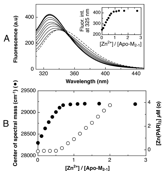
Figure 4. Apo- M_{2-1} \text{Zn}^{2+} uptake titration: (A) Apo- M_{2-1} (2 \mu\text{M} ) was titrated with increasing amounts of \text{ZnCl}_2 (ranging from 0 up to 5.4 \mu\text{M} ), and tryptophan fluorescence spectra were taken from each titration point. The dashed line represents the fluorescence spectrum of apo- M_{2-1} (0 \mu\text{M} \text{Zn}^{2+} ). Inset: Fluorescence intensity changes at 325 nm as a function of [\text{Zn}^{2+}]/[\text{apo-}M_{2-1}] . (B) Left axis: Tryptophan fluorescence CSM ( \bullet ) changes as a function of [\text{Zn}^{2+}]/[\text{apo-}M_{2-1}] . The CSM were calculated from the spectra shown in A. Right axis: titration of 100 \mu\text{M} PAR and 4 \mu\text{M} apo- M_{2-1} with increasing concentrations of \text{ZnCl}_2 . The formation of the \text{Zn}(\text{PAR})_2 complex ( \circ ) was monitored at 500 nm and plotted as a function of the [\text{Zn}^{2+}]/[\text{apo-}M_{2-1}] ratio. Each titration point was incubated for 5 min, and the experiment was performed at 20 ^\circ\text{C} .
