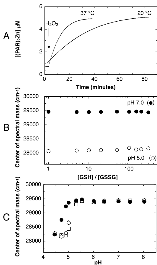
Figure 7. M 2-1 CCCH motif redox-state and pH dependence. (A) Oxidation of M 2-1 by hydrogen peroxide. M 2-1 without DTT at 6 μM was incubated with H 2 O 2 (3 mM) in sodium phosphate (pH 7.0) and 0.3 M NaCl at either 20 or 37 °C. Zinc release from M 2-1 upon oxidation was monitored over time at 500 nm, indicative of the formation of the Zn(PAR) 2 complex. (B) Tryptophan fluorescence CSM of M 2-1 as a function of GSH/GSSG ratios at either pH 7.0 (●) or pH 5.0 (○). Samples of M 2-1 at 6 μM were incubated for 16 h at 20 °C in 20 mM sodium phosphate at pH 7.0 or 20 mM sodium acetate at pH 5.0, both with 0.2 M NaCl and 5 mM final concentration of GSH/GSSG mixtures. (C) Tryptophan fluorescence CSM mass of M 2-1 at different pH values and GSH/GSSG ratios. M 2-1 at 6 μM was incubated for 16 h at 20 °C in broad range buffer (50 mM Tris-HCl, 25 mM MES, 25 mM sodium acetate, and 0.2 M NaCl) without glutathione (●) or with GSH/GSSG ratios of 1 (○), 100 (□), and 300 (Δ). The pH values of the solutions range from 4.4 to 8.4.
