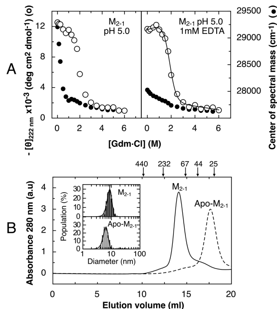
Figure 6. Gdm-Cl equilibrium unfolding of M 2-1 and apo-M 2-1 at pH 5.0 (A). M 2-1 (left graph) and apo-M 2-1 (right graph) equilibrium unfolding transition followed by monitoring changes in molar ellipticity at 222 nm (○) and tryptophan fluorescence CSM (●). The M 2-1 protein at 5 μM was incubated at 20 °C for 16 h in 20 mM sodium acetate (pH 5.0), 0.2 M NaCl, 1 mM DTT, and increasing Gdm-Cl concentrations. Apo-M 2-1 was prepared in each incubation tube by adding 1 mM EDTA. The two-state model fitting of apo-M 2-1 denaturation is plotted as a solid line. (B) Size exclusion chromatographies of M 2-1 (solid line) and apo-M 2-1 (dashed line) were carried out on a Superdex 200 column equilibrated in 20 mM sodium acetate (pH 5.0) and 0.2 M NaCl. Samples of M 2-1 (40 μM) were incubated at 20 °C for 2–3 h in 20 mM sodium acetate (pH 5.0), 0.2 M NaCl, and 1 mM DTT, with or without 1 mM EDTA. After the incubation period, the samples were subjected first to DLS measurements (inset) and then run on a S200 SEC. The positions of void volume (V 0 ), molecular size standards in kDa, and total volume (V 0 + V i ) are indicated above the graph. Inset: M 2-1 (above) and apo-M 2-1 (below) particle size distribution determined by DLS.
