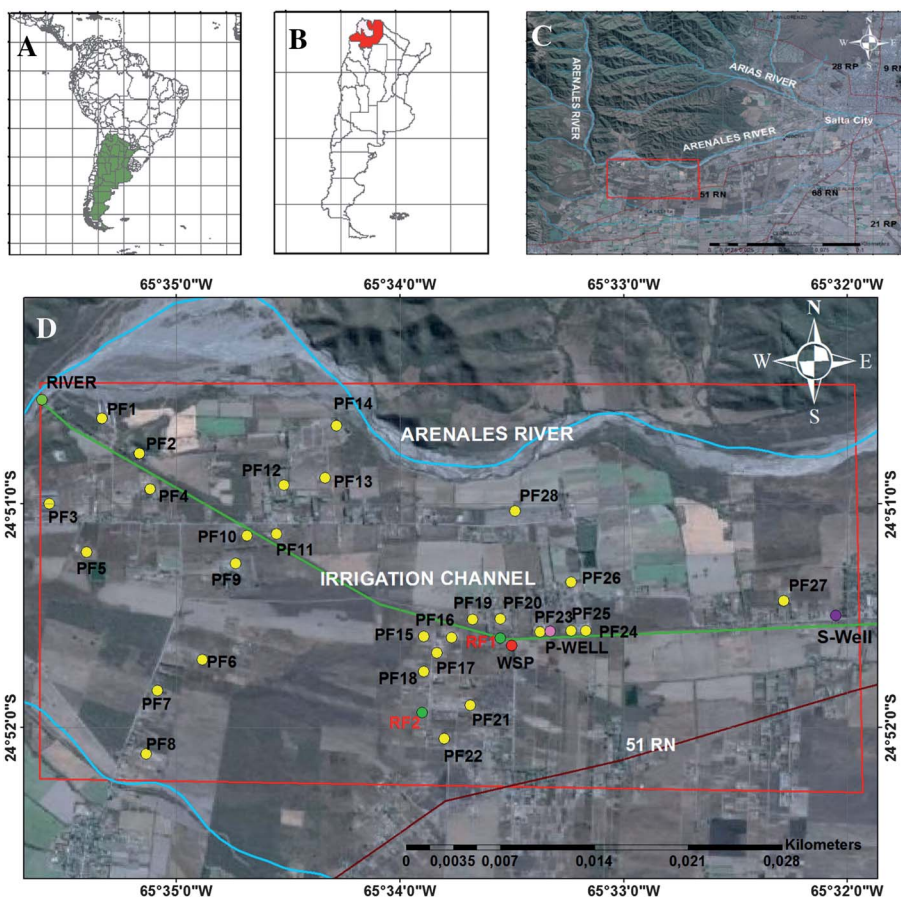
Fig. 1 Geographical location of the study area: (A) South America, (B) Argentina, (C) Salta province and (D) location of the poultry farms (PF) and shallow wells studied (RN: National Road; WSP: Wastewater Stabilization Pond; RF: Rearing Farming [swine]).
