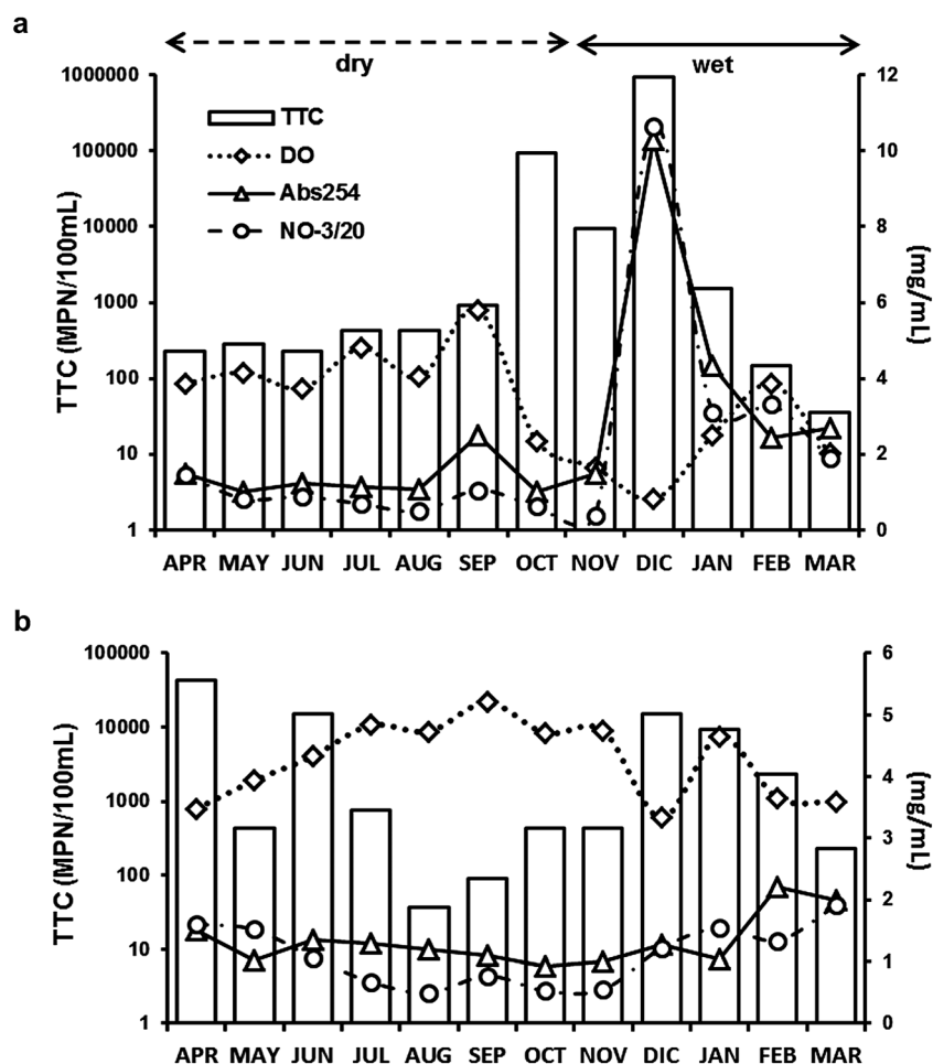
Fig. 4 Variation of thermotolerant coliforms (TTC), dissolved oxygen concentration (DO), natural organic matter ( Abs_{254} ), and nitrate concentration ( NO_3 ) along the monitoring year in shallow groundwater: (a) P-well and (b) S-well. The dry and wet seasons are indicated. Nitrate values were divided by 20 in order to fit them in the axis scale.
