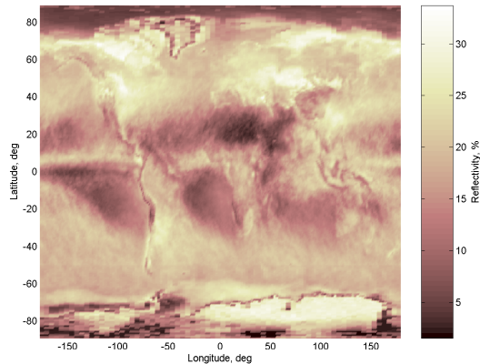
Figure 2. Plot of standard deviation of the TOMS reflectivity data recorded from January 1 to December 31, 2001.
