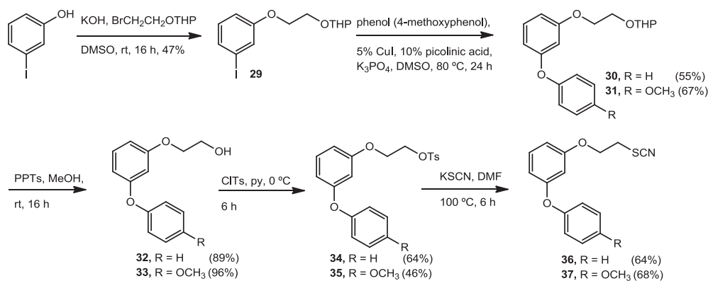
Scheme 6. Preparation of the regioisomers of WC-9 .
