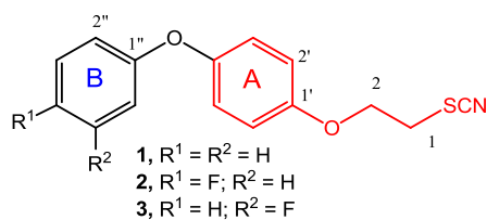
Fig. 1. Chemical structure of WC-9 (compound 1 ) and closely related analogs.
