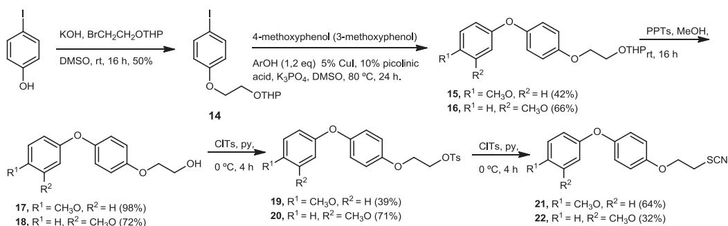
Scheme 4. Synthesis of methoxy derivatives of WC-9 at the B ring.
