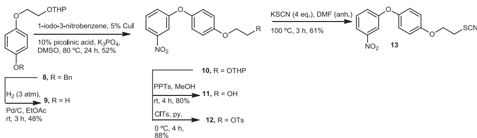
Scheme 3. Synthesis of the 2''-nitro derivative of WC-9 at the B ring.
