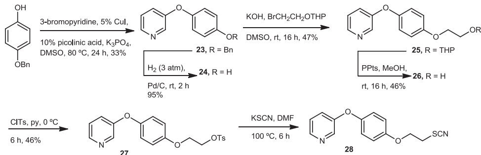
Scheme 5. Preparation of nitrogen-containing thiocyanates at the B ring.
