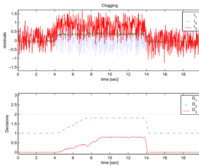
(b) Detection of the fault K_f clogging.
