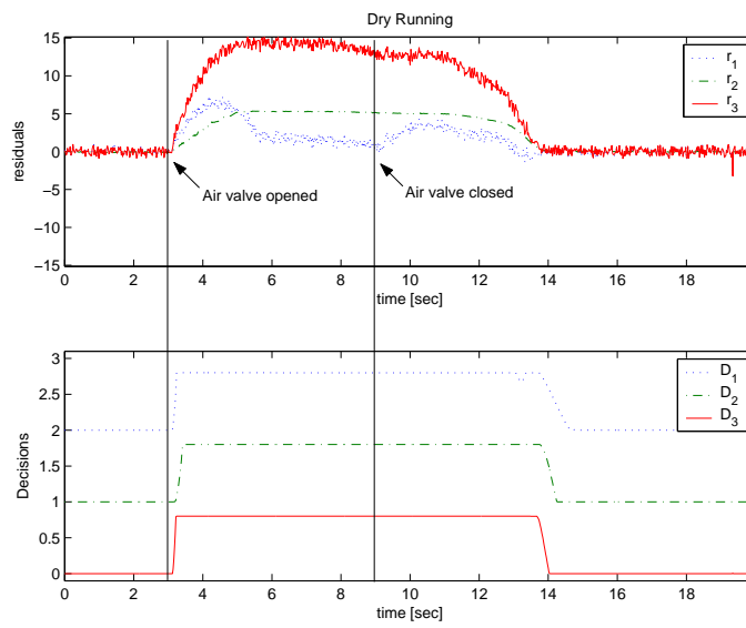
(b) Detection of the fault f_d dry running.
