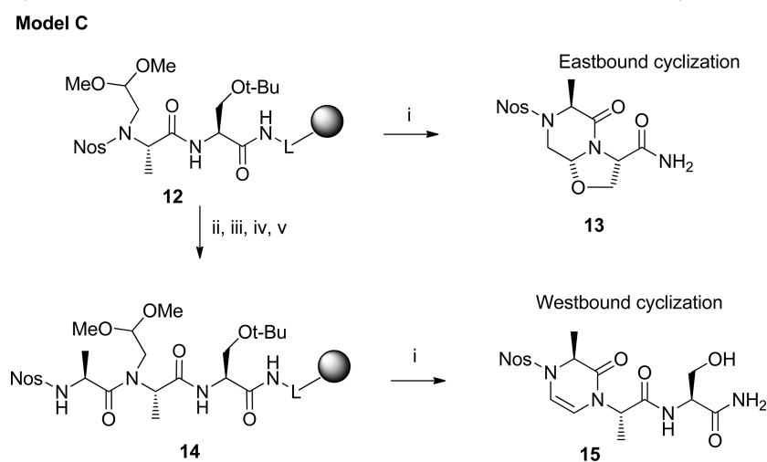
Scheme 7. Regioselectivity of Iminium Formation and Demonstration of Eastbound Viability a
