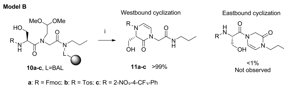
Scheme 6. Effect of the N -substituent on the Regioselectivity a
