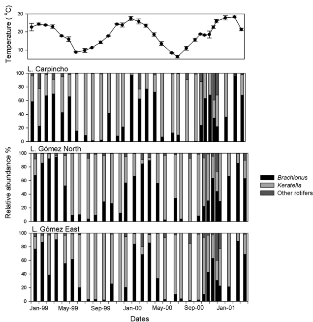
Fig. 3 Seasonal patterns of water temperature (upper panel) and relative abundance of the dominant genera of rotifers in L. Carpincho and L. Gómez (lower panels).
