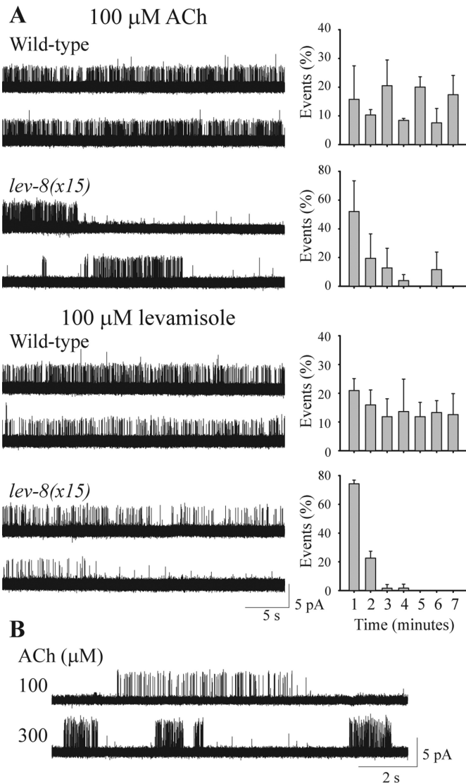
Fig. 4. Single-channel activity of L-AChRs lacking LEV-8 decreases significantly with time and occurs in clusters. A , left, continuous recordings from muscle cells derived from wild-type and lev-8(x15) mutant at 100 \mu\text{M} ACh or levamisole. Membrane potential, -100 mV. Filter, 9 kHz. Right, percentage of opening events per minute during the 7-min recording. B , Typical clusters of L-AChR lacking LEV-8 at 100 and 300 \mu\text{M} ACh.
