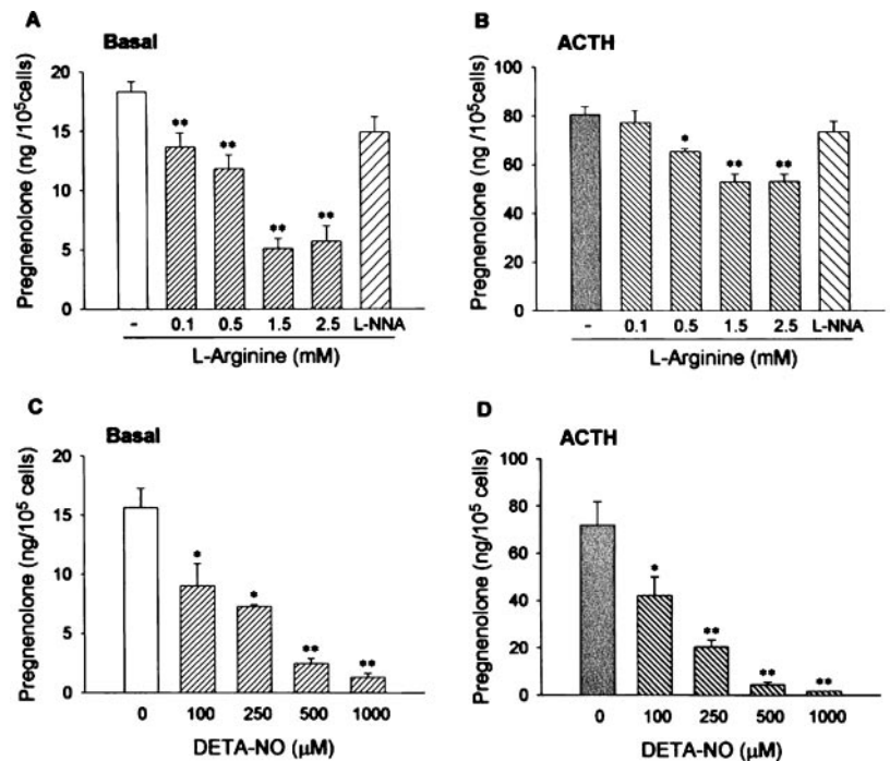
FIG. 7. Basal and ACTH-stimulated pregnenolone production by Y1 cells incubated in the presence of L-arginine or DETA-NO. Cells were preincubated for 15 min at 37^\circ\text{C} in the presence of cyanoketone ( 10 \mu\text{M} ), then incubated for 15 min with increasing concentrations of L-arginine ( 0.1 – 2.5 \text{ mM} ; A and B) or DETA-NO ( 100 – 1000 \mu\text{M} ) and further incubated for 2 h in the absence (A and C) or presence (B and D) of ACTH ( 0.2 \text{ mIU/incubation} ). When indicated, L-NNA ( 1 \text{ mM} ) was added together with cyanoketone 15 min before L-arginine ( 0.5 \text{ mM} ) addition. Pregnenolone production was assessed in the incubation medium by RIA. Each value represents the mean \pm SEM of three independent experiments, each performed in quadruplicate. *, P < 0.05 ; **, P < 0.01 ( vs. control, by Dunnett's t test).
