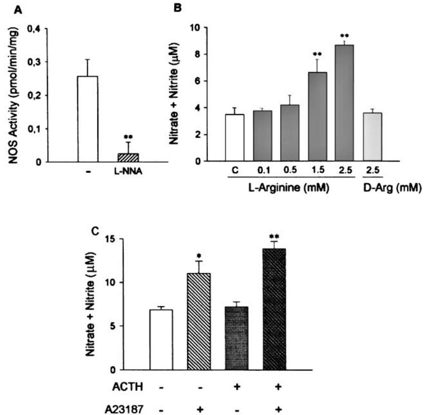
FIG. 6. L-Citrulline and nitrate plus nitrite levels in Y1 cells. A, Y1 cells homogenates were incubated for 60 min in the presence of 20 \mu\text{M} L- ^3\text{H} arginine with or without the addition of 1 \text{ mM} L-NNA as described in Materials and Methods . Values are the mean \pm SEM of three independent experiments, each performed in triplicate. **, P < 0.01 ( vs. control, by t test). B, Cells were incubated for 210 min at 37^\circ\text{C} in the presence of increasing concentrations of L-arginine ( 0.1 – 2.5 \text{ mM} ) or 2.5 \text{ mM} D-arginine as indicated. C, Cells were incubated for 210 min at 37^\circ\text{C} in the presence of 1 \text{ mM} L-arginine and 2 \text{ mM} \text{Ca}^{2+} with or without the addition of ACTH ( 10 \text{ mIU/incubation} ) and/or 10 \mu\text{M} A23187. Aliquots of the incubation medium were assayed for nitrate plus nitrite levels. Values in B and C are the mean \pm SEM of three independent experiments, each performed in triplicate. *, P < 0.05 ; **, P < 0.01 ( vs. control, by Dunnett's t test).
