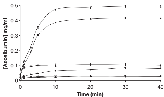
Fig. 3. Release of azo-BSA and sulfanilic acid adsorbed by beads using C. rugosa lipase. Symbols: \times and \blacksquare , sulfanilic acid and azo-BSA release from emulsan/alginate and alginate, respectively; \blacktriangle and \bullet , sulfanilic acid release from emulsan/alginate and alginate beads, respectively; * and \blacklozenge , sulfanilic acid and azo-BSA release from emulsan/alginate and alginate beads, respectively, incubated without lipase.
