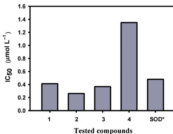
Figure 4. Results of in-vitro SOD-mimic activity testing for 1–4 with the native bovine Cu,Zn-SOD*, expressed as IC 50 (µmol L -1 ). *Extracted from reference [23].
