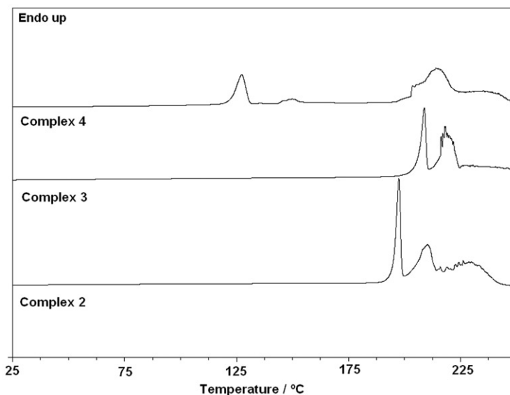
Figure 2. DSC analysis for powdered [\text{Cu}_2(\text{fen})_4(\text{L})]_n complexes ( \text{L} = 4,4' -bipy (2), pyz (3), and 2,5- \text{Me}_2\text{pyz} (4)) under \text{N}_2 flux ( 20 \text{ cm}^3 \text{ min}^{-1} ). Heating rate: 5^\circ\text{C min}^{-1} .
