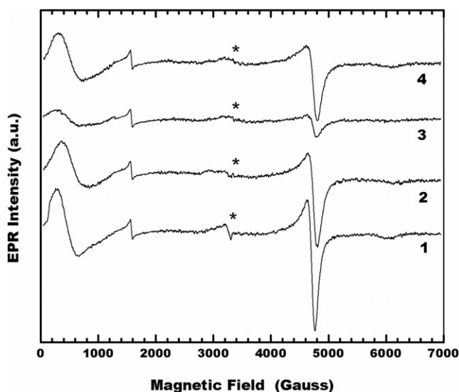
Figure 1. X-band EPR spectra of powdered dinuclear complexes [\text{Cu}_2(\text{fen})_4(\text{dmf})_2] ( 1 ), [\text{Cu}_2(\text{fen})_4(4,4'\text{-bipy})_n] ( 2 ), [\text{Cu}_2(\text{fen})_4(\text{pyz})_n] ( 3 ), and [\text{Cu}_2(\text{fen})_4(2,5\text{-Me}_2\text{pyz})_n] ( 4 ) at room temperature asterisk (*) denotes small signals due to monomeric impurities.
