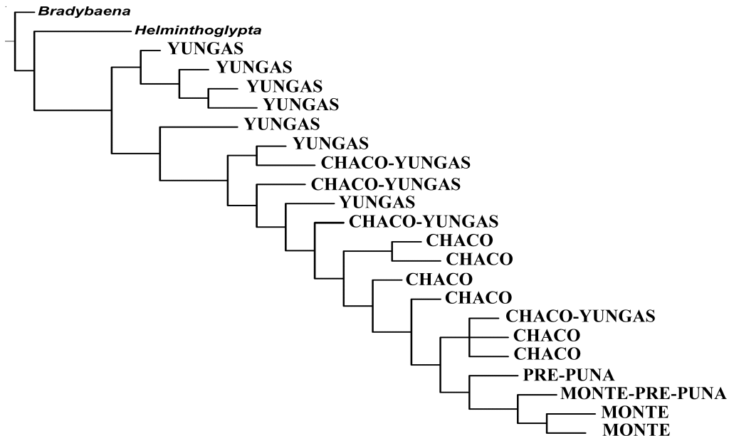
FIG. 24. Area cladogram of the Epiphragmophora species studied based on the preferred cladistic hypothesis obtained (Fig. 23).
