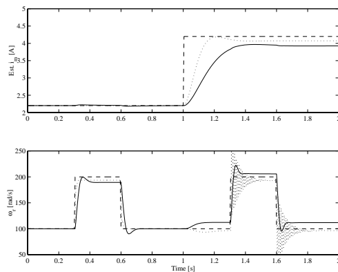
Figure 5: Simulation of the controlled system. The plot shows the reference signal (---), the non-robustly controlled system ( \cdots ) and the robustly controlled system (—).
