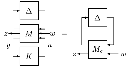
Figure 2: The interconnection of the nominal system M , the uncertainty block \Delta , and the controller K .
