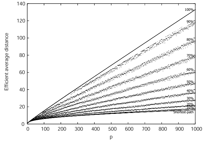
Figure 12. Efficient average distances using RS2, varying x_{avg} .
