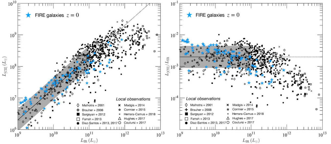
Figure 6. The L_{[\text{C II}]} versus L_{\text{IR}} (left panel) and the L_{[\text{C II}]} / L_{\text{IR}} versus L_{\text{IR}} (right panel) relations of z = 0 galaxies. In the two panels, filled cyan stars show the result of the FIRE galaxies, whereas black symbols indicate the observational data from different studies, including Malhotra et al. (2001, diamond), Brauher et al. (2008, crosses), Sargsyan et al. (2012, filled squares), Farrah et al. (2013, empty squares), Díaz-Santos et al. (2013, 2017, filled circles), Magdis et al. (2014, ‘X’s), Cormier et al. (2015, empty stars), Herrera-Camus et al. (2018, asterisks), Hughes et al. (2017, triangles), and Coutursi et al. (2017, empty circles). Observations show that L_{[\text{C II}]} / L_{\text{IR}} ratio of galaxies is nearly a constant at 10^9 \lesssim L_{\text{IR}} \lesssim 10^{11} L_{\odot} , but declines with L_{\text{IR}} at L_{\text{IR}} \gtrsim 10^{11} L_{\odot} . In the two panels, black line (solid at L_{\text{IR}} < 10^{11} L_{\odot} and dotted at L_{\text{IR}} \geq 10^{11} L_{\odot} ) indicates the median L_{[\text{C II}]} / L_{\text{IR}} ratio ( \approx 2 \times 10^{-3} ) of the galaxies having L_{\text{IR}} < 10^{11} L_{\odot} and grey-shaded bar indicates the 1\sigma scatter of the L_{[\text{C II}]} / L_{\text{IR}} ratio of these galaxies. FIREBOX successfully reproduces the observed L_{[\text{C II}]} versus L_{\text{IR}} (and the L_{[\text{C II}]} / L_{\text{IR}} versus L_{\text{IR}} ) relation at z = 0 .
