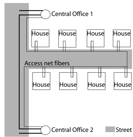
Figure 2. Proposed FTTH-wiring, ensuring physical redundancy. Compared to Figure 1, each house is now provided with a double wiring and connected to two Central offices.
