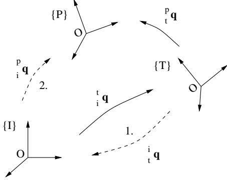
Fig. 7: Transformations used in calculating the error quaternion {}^p_t\mathbf{q} .
