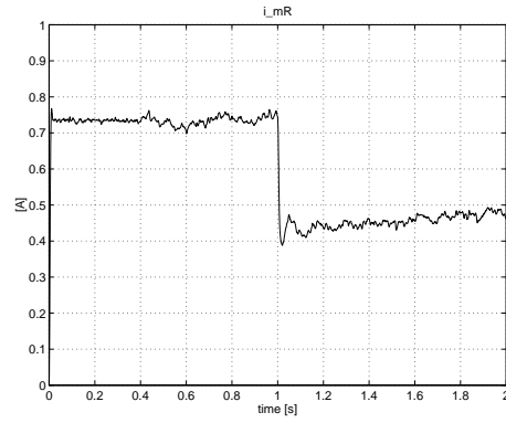
b) Estimated magnetizing current i_{mR} (experiment)
