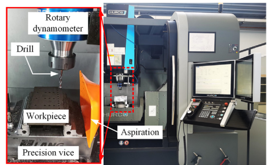
Fig. 2. Experimental set-up.
