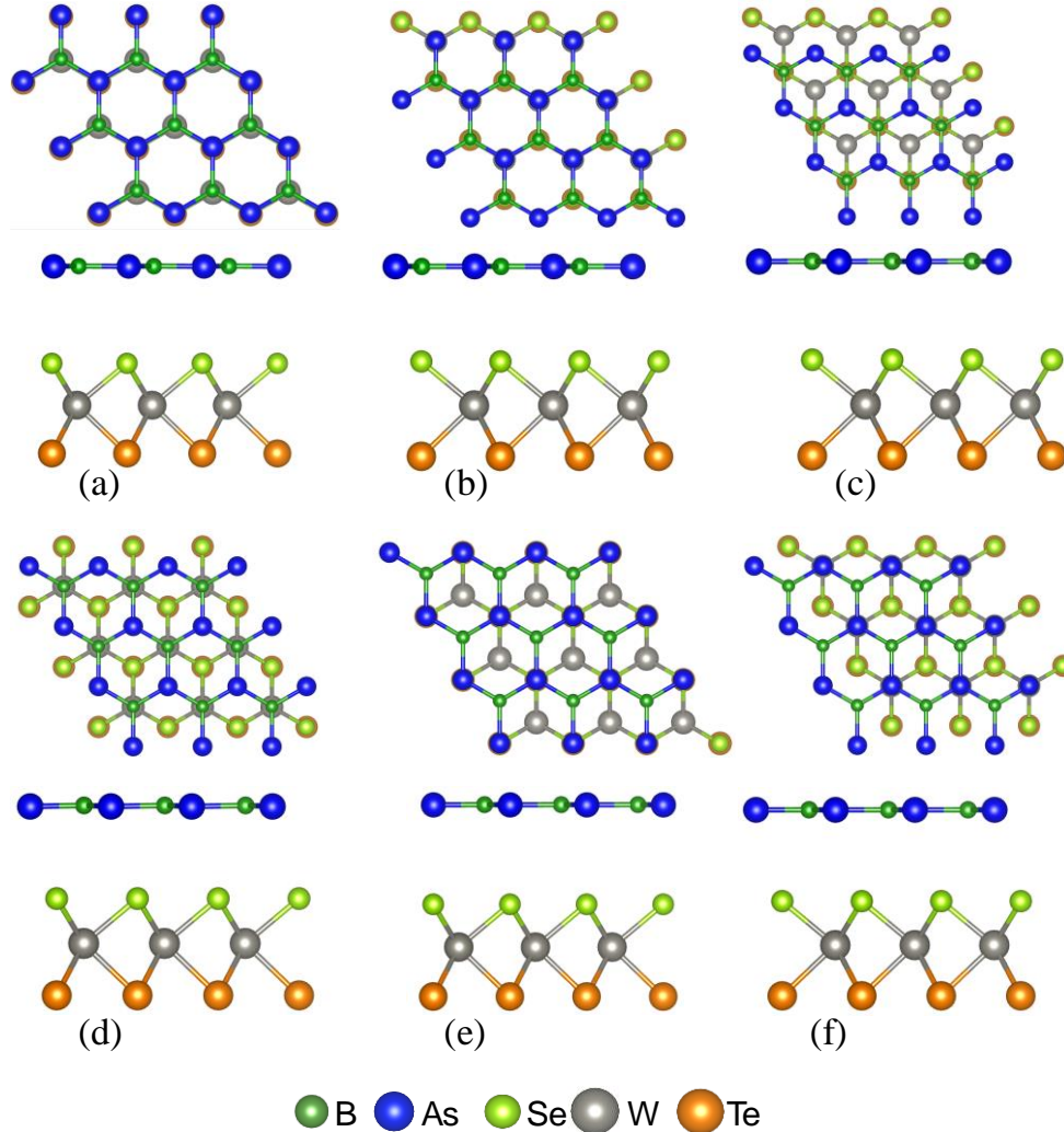
Figure 1: Top and side views of different configurations of vdWHs obtained from the stacking of BAs and Janus-WSeTe: (a) stacking-A, the B and As atom sits on the top of W and Se atom, respectively; (b) stacking-B, the B and As atom sits on the top of Se and W atom, respectively; (c) stacking-C, the As atom is on the hollow site of the hexagonal, the B atom occupies the top of Se atom); (d) stacking-D, the As atom is on the hollow site of the hexagonal, the B atom occupies the top of W atom, respectively; (e) stacking-E, the As atom sits on the top of Se atom, while the B atom is on the center of the hexagonal site; (f) stacking-F, the As atom sits on the top of W atom, while the B atom is on the center of the hexagonal site, BAs/Janus WSeTe vdW heterostructure. The BAs/Janus WTeSe vdWHs are formed by swapping the positions of Se and Te atoms in the six configurations (a-f) . The color scheme for each atom is given at the bottom.
