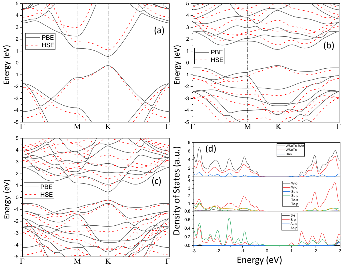
Figure 3. The band structures of (a) BAs, (b) Janus WTeSe, (c) H-I heterostructure computed using the PBE (black solid lines) and HSE06 (red dashed lines) functionals. (d) Density of states of the H-I heterostructure.
