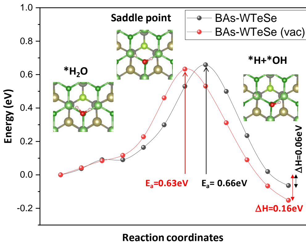
Figure 7. Reaction profiles for the water splitting on BAs-WTeSe without Te vacancies (black line) and BAs-WTeSe with Te vacancies (vac) (red line).
