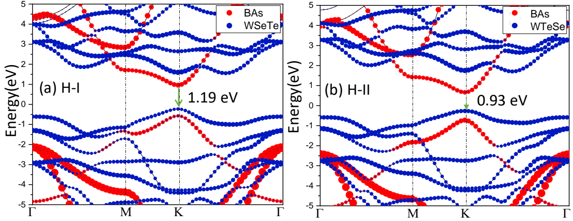
Figure 4. Projected band structures of the (a) H-I and (b) H-II heterostructures.
