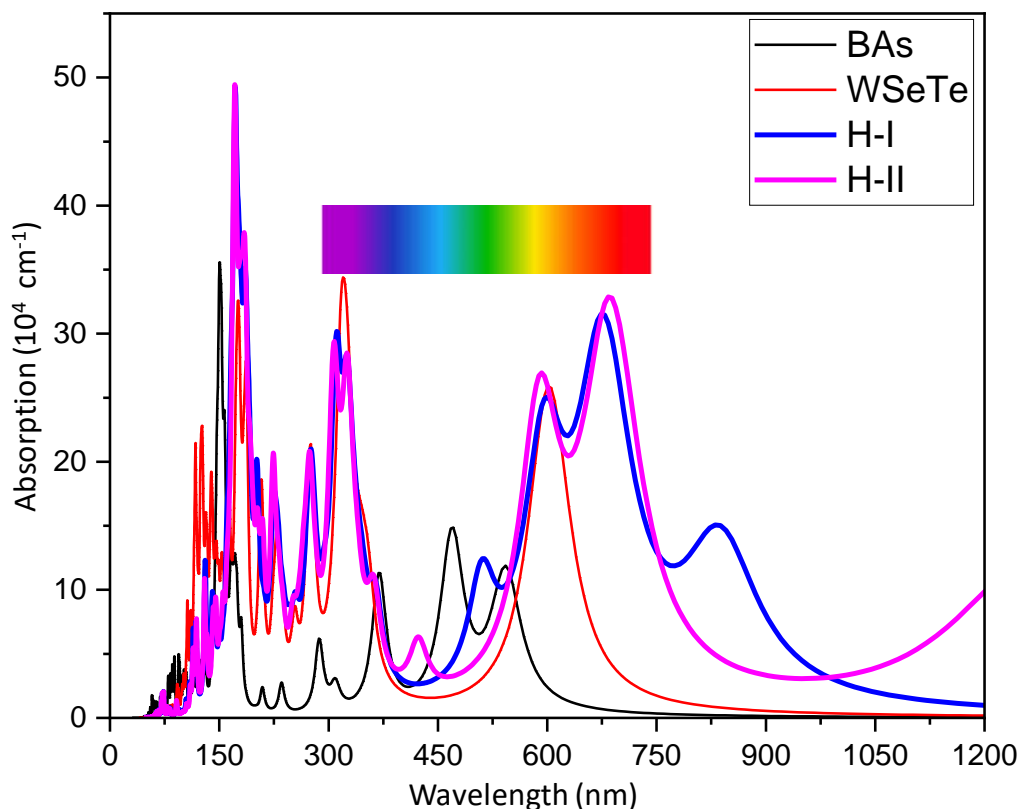
Figure 8. The absorption coefficient of the monolayers BAs, WSeTe, and two different heterostructures.
