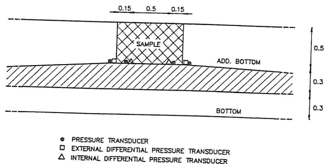
Fig. 1 Test section.
