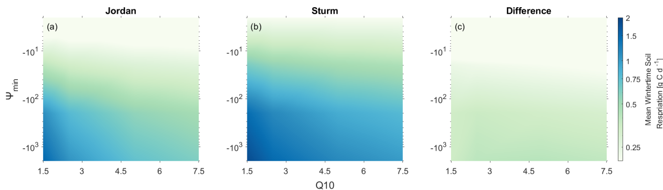
Figure 3. Contour plots showing the relative influence of \Psi_{\min} and Q10 on the simulations of mean soil respiration for all three snow-covered non-growing seasons using the snow thermal conductivity parameterisations of (a) Jordan (1991) and (b) Sturm et al. (1997). The difference between the two snow thermal conductivity parameterisations is shown in (c).
