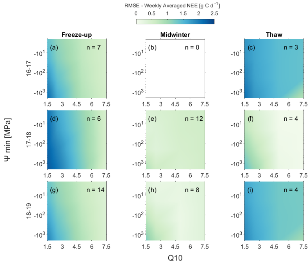
Figure 4. Evaluation of the impact of \Psi_{\min} and Q10 parameterisations on simulated net ecosystem exchange (NEE) during freeze-up (a, d, and g), midwinter (b, e, and h), and thaw (c, f, and i) periods of each snow-covered season for simulations using the Sturm et al. (1997) snow thermal conductivity parameterisation. The number of weekly averages included in each panel are denoted by n values.
