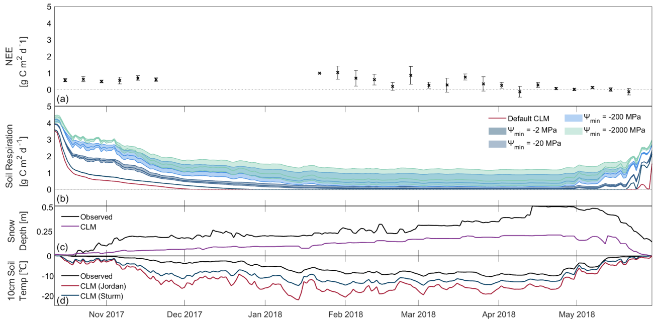
Figure 1. (a) Mean (crosses) and uncertainty (as per Lasslop et al. (2008); error bars) of measured NEE at weekly intervals. (b) Simulated soil respiration. The default simulation (red) uses the Jordan (1991) parameterisation of snow thermal conductivity, and blue colours represent simulations using the Sturm et al. (1997) parameterisation of snow thermal conductivity. Darker blue colours represent less-negative \Psi_{\min} values and paler blue colours represent more-negative values of \Psi_{\min} . Shaded areas in panel (b) represent the range of respiration fluxes for simulations using the Sturm et al. (1997) snow thermal conductivity and the same \Psi_{\min} but with different values of Q10 (1.5, 2.5, 5.0, 7.5). (c) Observed (black) and simulated (purple) snow depths. (d) 10 cm soil temperatures, both observed (black) and simulated using both the default Jordan (1991; red) and Sturm et al. (1997; blue) snow thermal conductivity parameterisations.
