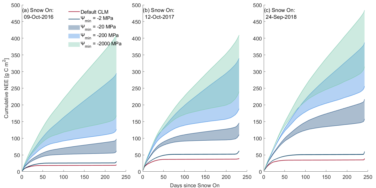
Figure 2. Cumulative net ecosystem exchange (NEE) for the simulated snow cover duration of (a) 2016–17 (227 d), (b) 2017–18 (231 d), and (c) 2018–19 (242 d) from the ensemble of simulations. Blue colours represent simulations using the snow thermal conductivity parameterisation of Sturm et al. (1997), with darker colours for less-negative \Psi_{\min} . The shaded areas represent the range of Q10 (1.5–7.5) for each \Psi_{\min} . The dark red line represents the default CLM snow thermal conductivity parameterisation of Jordan (1991).
