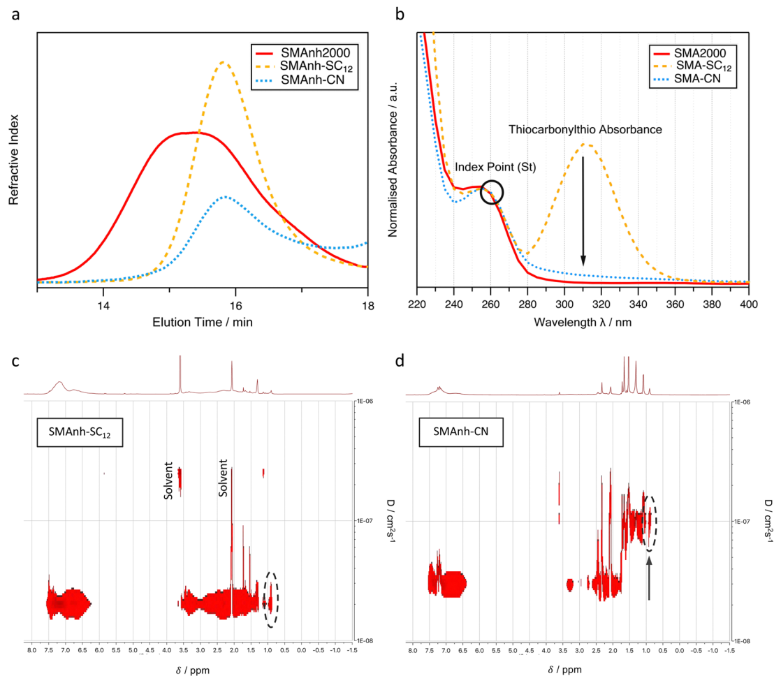
Fig. 3 (a) GPC chromatograms for SMAh2000, SMAh-SC 12 and SMAh-CN. (b) UV-vis spectra of SMA-SC 12 and SMA-CN in PBS solutions normalised at styrene absorbance (260 nm) for comparison. (c-d) 1 H DOSY NMR spectra of (c) SMAh-SC 12 and (d) SMAh-CN. Arrow indicates cleavage of thiocarbonylthio end group which diffuses at the rate of the copolymer in SMAh-SC 12 , and at the rate of the solvent in SMAh-CN.
