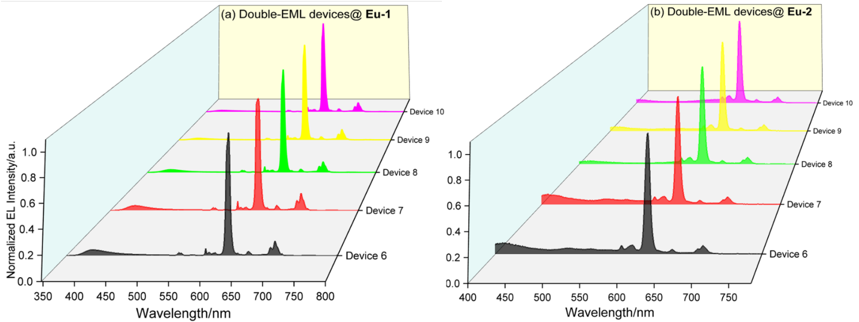
Figure 9: Normalized EL spectra of double-EML devices of Eu-1 and Eu-2 at different doping concentrations operating at J = 10 \text{ mA/cm}^2 .
