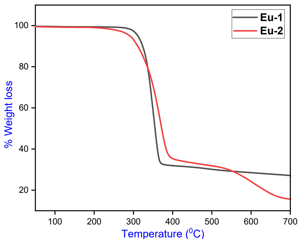
Figure 7: Thermograms of Eu-1 and Eu-2 under a N 2 atmosphere.
