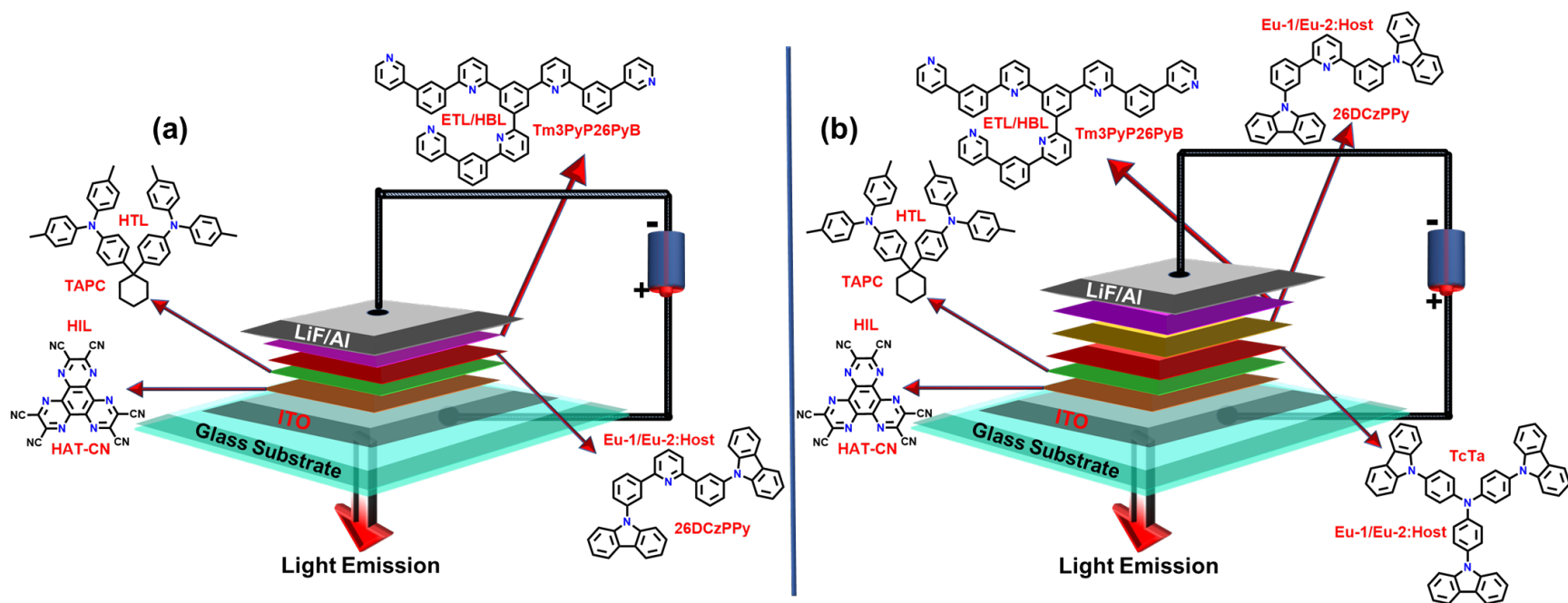
Figure 8: General device configuration (a) single-EML and (b) double-EML OLEDs (where = HIL: Hole Injection Layer; HTL: Hole Transport Layer; ETL: Electron Transport Layer; HBL: Hole Blocking Layer; HAT-CN: 1,4,5,8,9,11-hexaazatriphenylene hexacarbonitrile; TAPC: Di-[4-(N,N-ditolyl-amino)-phenyl]cyclohexane; Tm3PyP26PyB: 1,3,5-Tris(6-(3-(pyridin-3-yl)phenyl)pyridin-2-yl)benzene; Host : (26DCzPPy: 2,6-bis(3-(9H-carbazol-9-yl)phenyl)pyridine; TcTa: 4,4',4''-Tris(carbazole-9-yl)triphenylamine). Specific details of the different composition are included the ESI.
