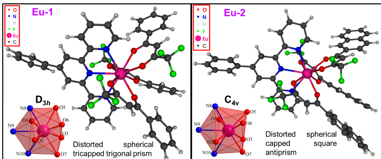
Figure 2: Geometry of Eu-1 and Eu-2 complexes calculated at the PBE1PBE/TZVP/MWB52 level of theory.
