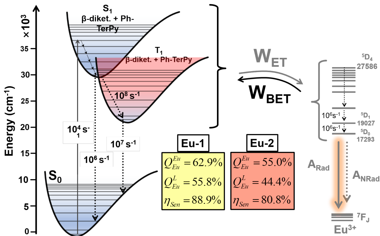
Figure 6: Jablonski diagram showing the states included in the process of ET of the complexes.
