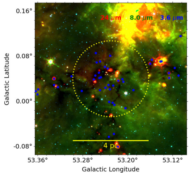
Figure 14. Multiwavelength colour-composite image of a hub-filament system in IRDC G53.2. The dots represent the MHOs identified in this study. The dotted circle indicates the central region of the hub-filament system.
