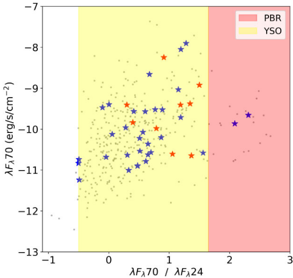
Figure 3. Plot of 70 \mu\text{m} flux as a function of the ratio of 70 to 24 \mu\text{m} flux. HOPS protostars (Manoj et al. 2013; Stutz et al. 2013) are shown as grey dots. The blue stars are the YSOs identified in this study, having detection in IRAC bands. Deeply embedded sources lacking detection in the IRAC bands are plotted as red stars. The yellow shaded region corresponds to \log\left(\frac{\lambda F_{\lambda 70}}{\lambda F_{\lambda 24}}\right) > -0.5 which is used as the colour criterion for YSO identification. The red shaded regions represent PBRs, i.e. sources with \log\left(\frac{\lambda F_{\lambda 70}}{\lambda F_{\lambda 24}}\right) > 1.65 .
