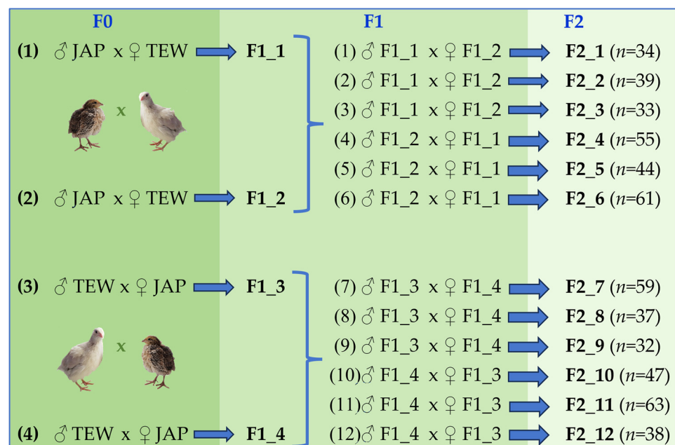
Figure 3. Overview of the experimental design. The reference population consisting of 146 F 2 male quails was created and extensively phenotyped using reciprocal crosses between a slow-growing Japanese and a fast-growing Texas White breed. n , number of progenies (of both sexes) from each F 2 family.
