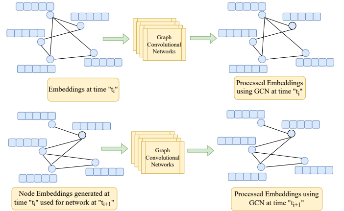
Fig. 3. Processing the features of the nodes iteratively using GCN. The features of the nodes from the previous timestamp are used as the inputs for the current network structure and the embeddings are processed using the GCN architecture. The output of the first step forms the input of the second step.
