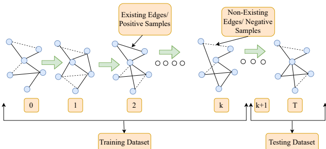
Fig. 1. Splitting of the entire temporal dataset by keeping 80% dataset for training dataset and the remaining for 20% for testing dataset.
