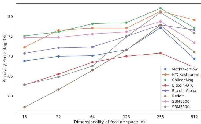
Fig. 5. Dimensionality of feature space (d) vs. Accuracy for various datasets.
