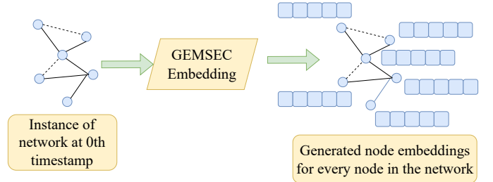
Fig. 2. Generating the initial features for the network's node using GEMSEC embedding. The network structure at the first timestamp is used to generate the embeddings. Here, the connected circles refer to the state of the network at the first timestamp. The circles represent the nodes while the lines represent the edges. The array of squares shows the node embeddings for each node in the network.
