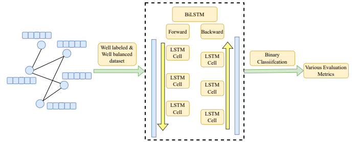
Fig. 4. Using a well-labeled and well-balanced dataset with embeddings as features and existence and non-existence of edges as labels dataset, for link prediction using the BiLSTM model.
