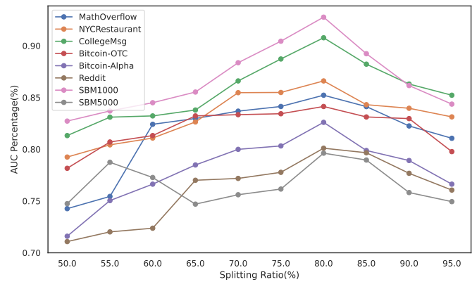
Fig. 6. AUC values obtained by our algorithm as the value of the splitting ratio for the dataset is varied on all the datasets.
