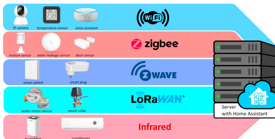
Fig. 1. Architecture of multi-layer integration of wireless protocols.
