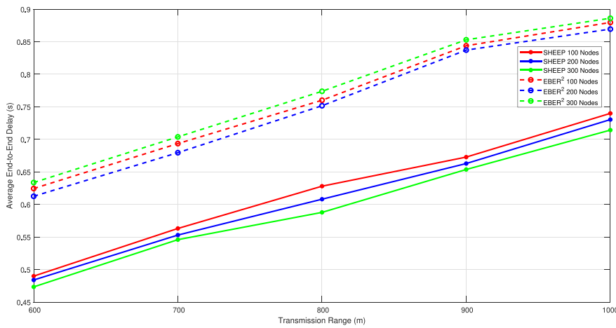
Fig. 21. The effect of transmission range on end-to-end delay.
