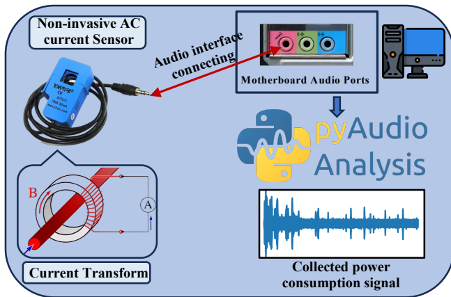
Fig. 2. Current Transformer and its audio interface.
