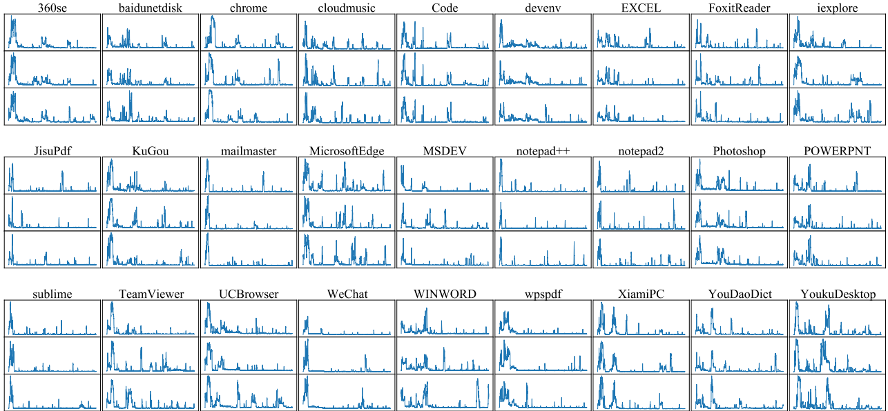
Fig. 7. Power curves for several applications during startup. For a specific application, the power curves during initialization are not exactly the same but similar; whereas for different applications, they start at different speeds and duration. Therefore, the power curves during initialization are different.
