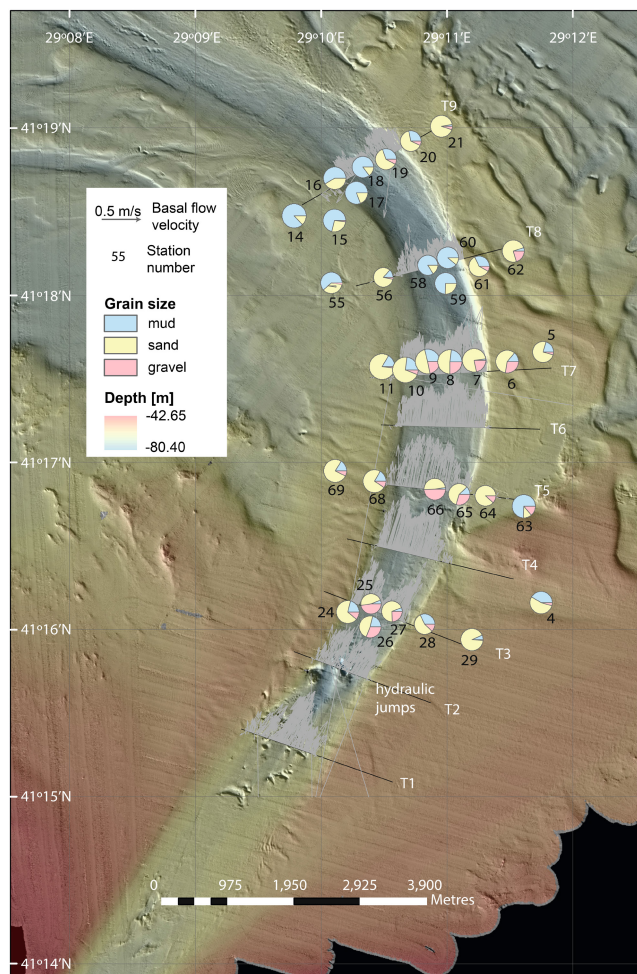
FIGURE 5 Near-bed flow velocities in relation to bed material size. Grey arrows represent the three-dimensional flow velocity at a height of 3 m over the sea floor ( Z/H \sim 0.1 ). Black numbers represent grab sample station.
