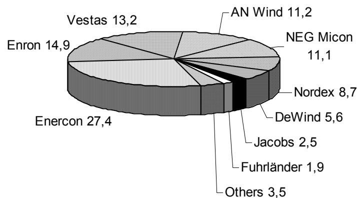
Figure 3. Shares of the suppliers on the German market in % of the installed rated power in 2000. Source: Rehfeldt, Knud: Wind Energy Use in Germany – Status 31.12.2000.
