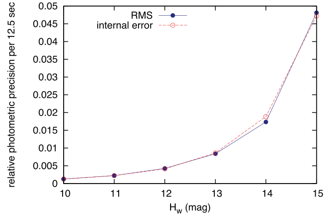
Fig. 17. Estimation of the uncertainties per single exposure of 12.5 s as a function of the magnitude of the stars. Red circles connected with the dashed line labeled as “internal error” present the photometric errors computed from the Poisson noise and the readout noise. The solid blue circle connected with the blue line labeled with “RMS” shows the photometric errors computed from the RMS error of the photometric measurement of 100 simulated images for each brightness of a star created with JIS (sub-subsection 3.6.2).
