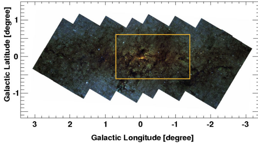
Fig. 2. Planned survey area of the JASMINE GCS program (highlighted with a yellow open square) overlaid on the image of the SIRIUS survey (Nishiyama et al. 2006).
