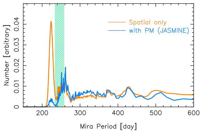
Fig. 5. Expected period distribution of the Mira variables in the NSD of the simulation shown in figure 4. The periods of Miras are derived from the age of star particles in the simulation snapshot at t = 5 Gyr, using the empirical age–period relation in Grady, Belokurov, and Evans (2019). The orange line indicates the period distribution of Miras, when the star particles are chosen by spatial information only, i.e., by the location corresponding to the galactic longitude and latitude range of the NSD. The blue line shows the period distribution when the stars are selected by the galactic longitude and latitude region of the NSD and the line-of-sight velocity and proper motion region corresponding to the NSD kinematics. In this simulation snapshot, the bar age is 3.5 Gyr (green shaded region). Here, we have assumed that there is a kinematically hot component, i.e., a classical bulge, which is 1 Gyr older than the formation age of the bar. The orange line shows significant contamination from such a component, while the blue line with the additional kinematical selection of the NSD shows a sudden decrease of the population with shorter periods than about 250 d, which corresponds to the formation age of the bar.
