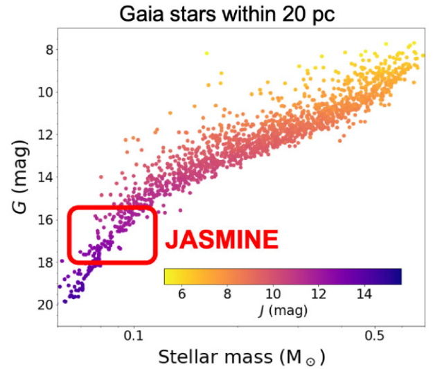
Fig. 13. Gaia G -band ( y -axis) and 2MASS J -band (colors) magnitudes of the stars within 20 pc as a function of the stellar mass ( x -axis). The UCD region to which JASMINE is sensitive to planets comparable to or higher than Gaia is indicated by the red box.
