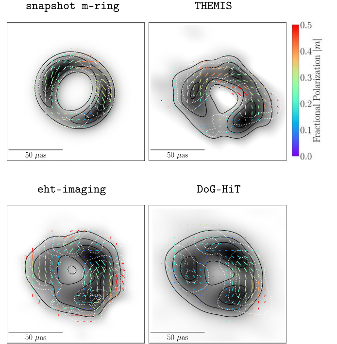
Figure 9. Polarimetric images of Sgr A* from Figure 8, but with EVPAs rotated by 46.0 deg to account for the median Faraday rotation in the combined April 6 and 7 data set (Table 5). The color-bar range is fixed for all panels.
