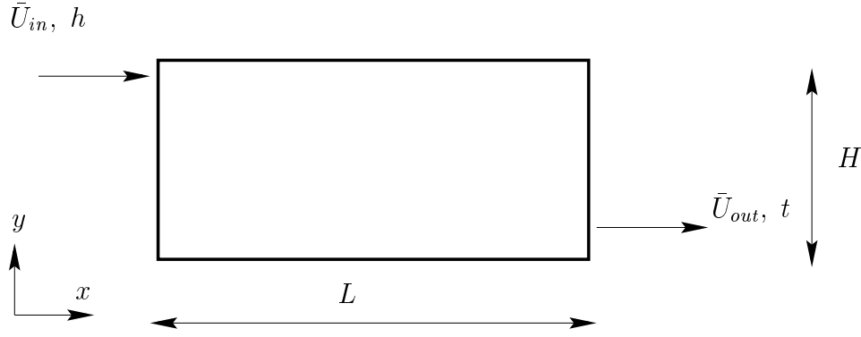
Figure 2: Configuration. L = 3H , h/H = 0.01 , t/H = 0.15 . Re = \bar{U}_{in}h/\nu = 7000 .
