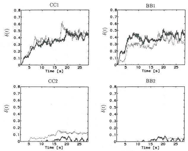
Figure 4: 2-storey frame. Estimated local damages with \beta_0 = 0.8 m/s 3/2 . [—]: Present method, [···]: SARCOF.
