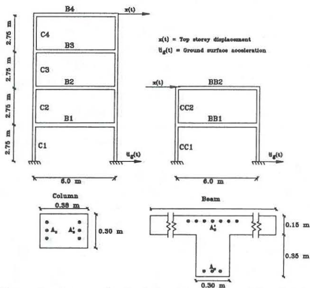
Figure 1: Linear-elastic finite element models of reinforced concrete frames.
