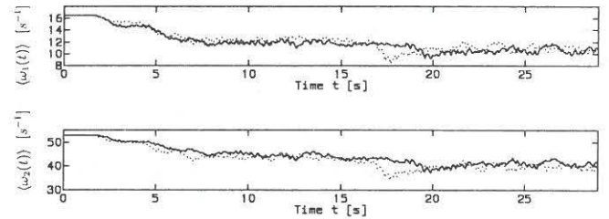
Figure 5: 2-storey frame. Comparison of reproduced eigenfrequencies. [—]: Measured eigenfrequencies, [···]: SARCOF. \beta_0 = 0.8 m/s 3/2 .
