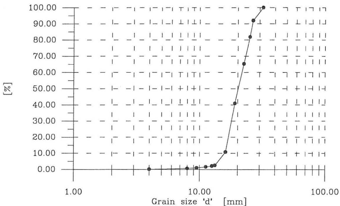
Figure 2 Grain size distribution for Portland gravel 16-32 mm.
