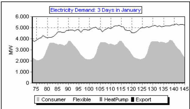
Diagram 12: Example of flexible demand
