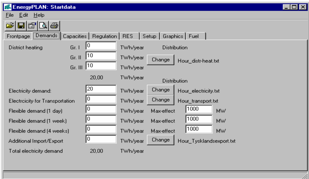
Diagram 3 : Demands input data window
