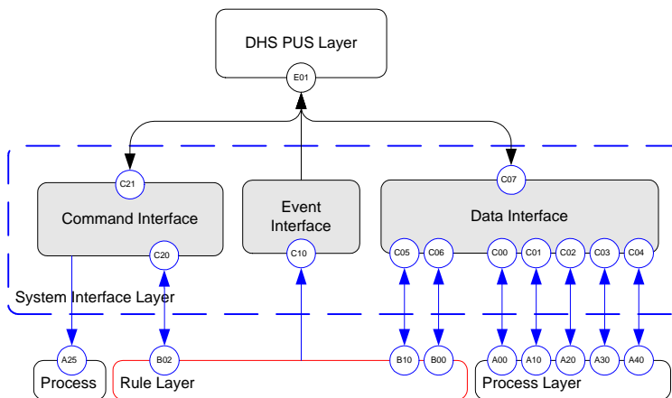
Fig. 3.3: System Interface Layer architecture. Interfaces to Rule Layer and Process Layer are indicated. [3]
