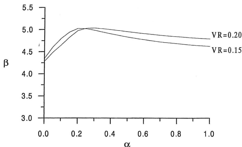
Figure 11.1. Reliability index for environmental load.
