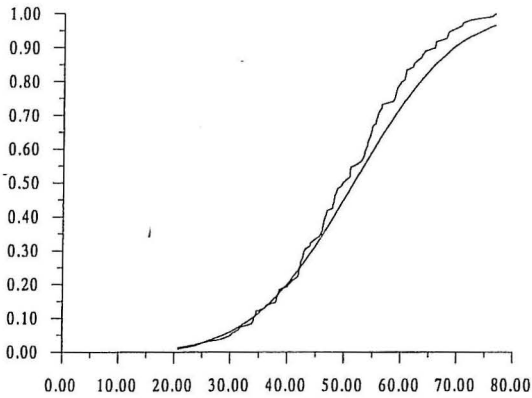
LT30: \kappa =15% truncation
