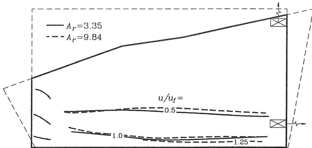
Fig. 3. Normalized velocity distribution versus Archimedes' number.
