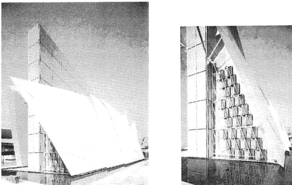
Fig. 1. a) The Danish Pavilion at the World Exposition EXPO '92 in Seville. b) Cooling elements in the south gable.
