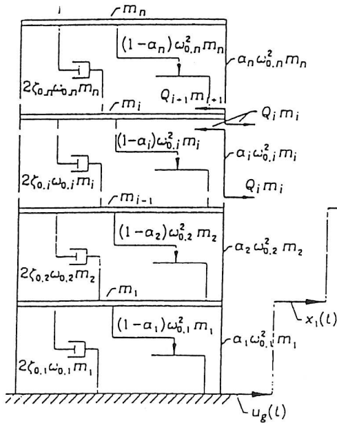
Figure 2. MDOF shear frame with local hysteretic oscillators.
