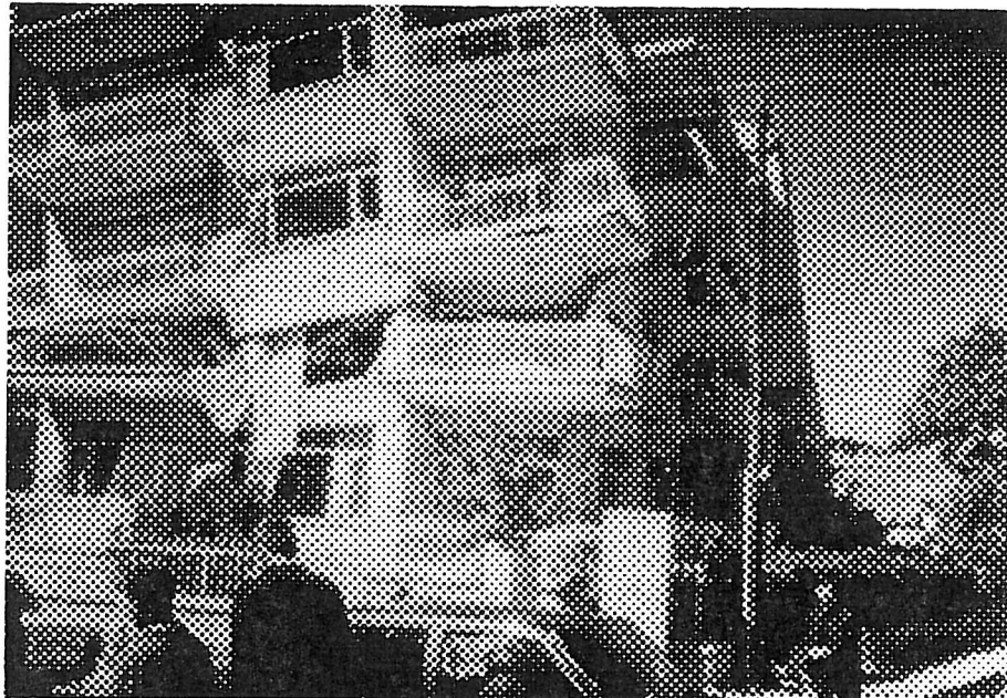
Figure 1. Collapse of an intermediate floor due to the October 1995 Earthquake, Dinar, Turkey. (Photograph taken by Prof. Hasan Bodurođlu of İstanbul Technical University, Turkey).
