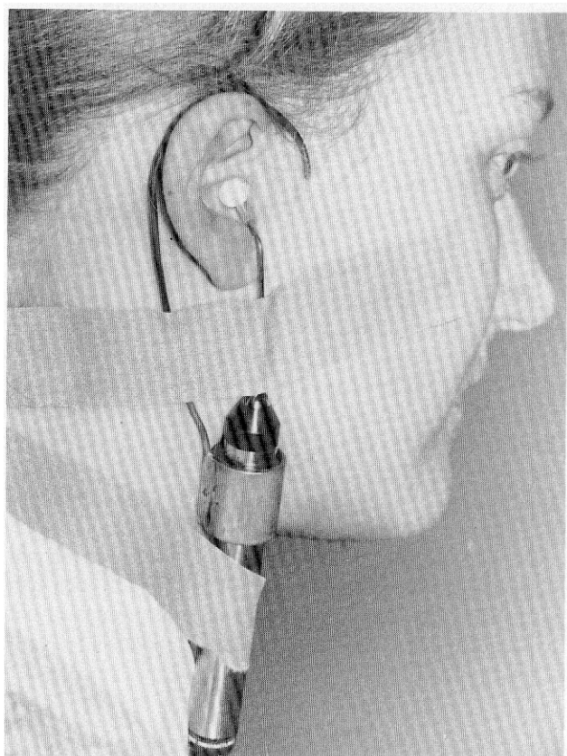
Fig. 3. Probe microphone mounted on subject to measure blocked ear canal pressure P_5 .
