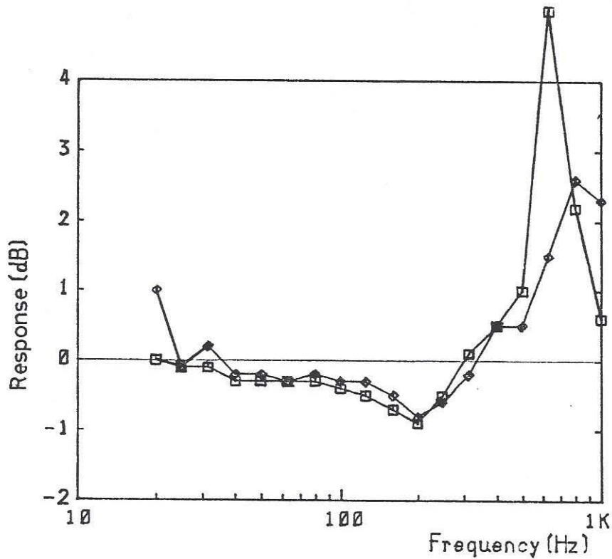
Figure 5. Difference of the sound level at the pinna and at the head position without subject. Measured at the head and torso simulator placed on a small chair ( \diamond ) or a big chair ( \square ) and 8 loudspeakers as sound source.
